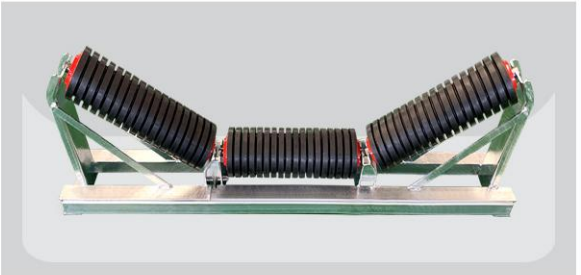
Impact Idler 缓冲托辊组
